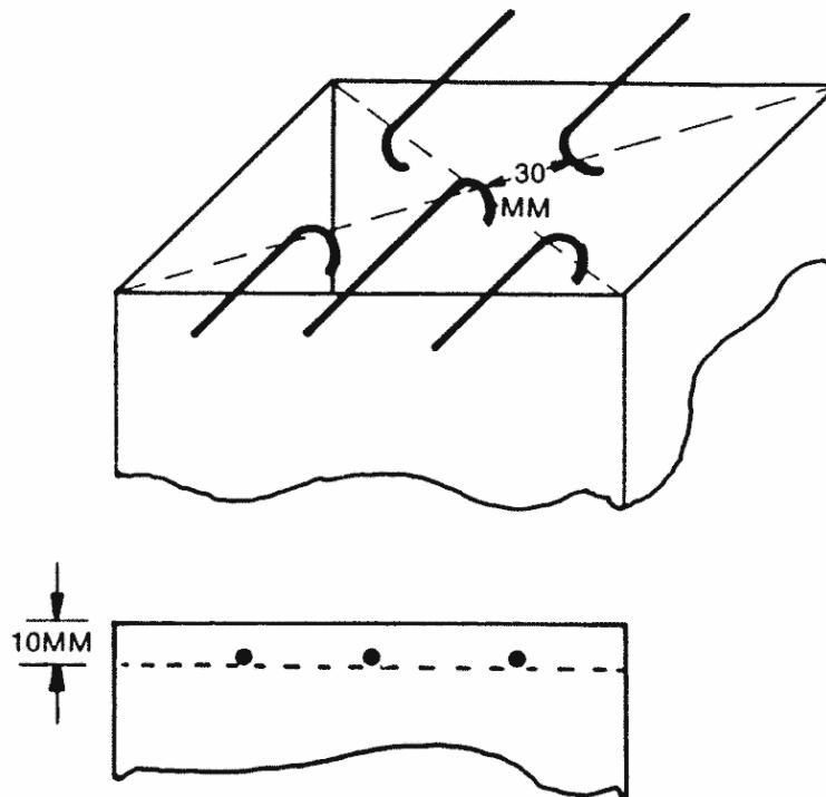
Figure 5. Thermocouple Position
