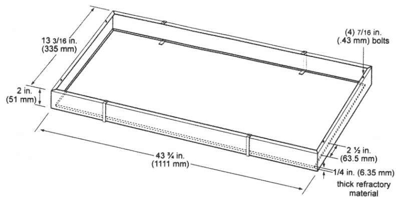
Figure 4 - Sliding Platform
