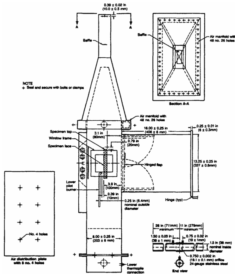
Figure 1B Rate of Heat Release Apparatus
