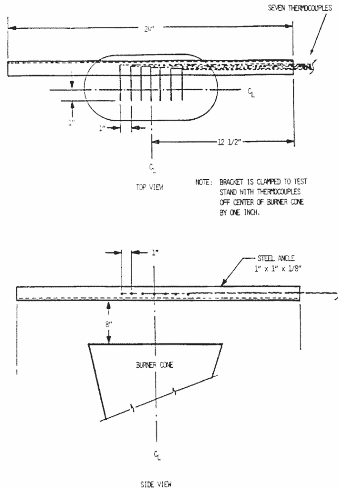
FIGURE 3. THERMOCOUPLE RAKE BRACKET
