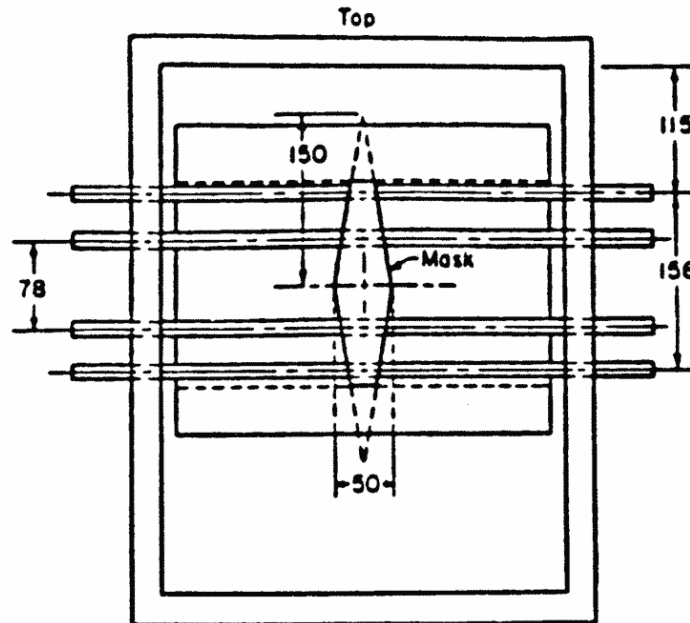
Figure 1B Rate of Heat Release Apparatus
