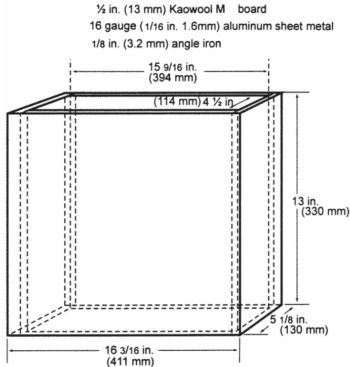
Figure 2 - Internal Chimney
