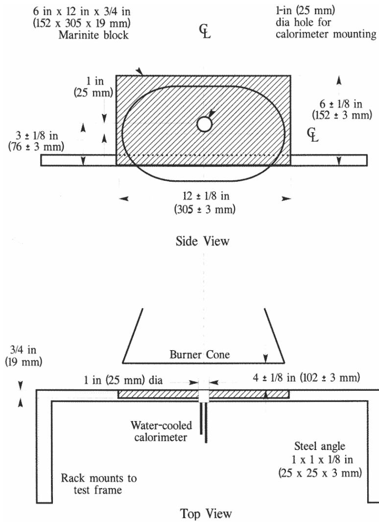
Figure 4 - Calorimeter Position Relative to Burner Cone
