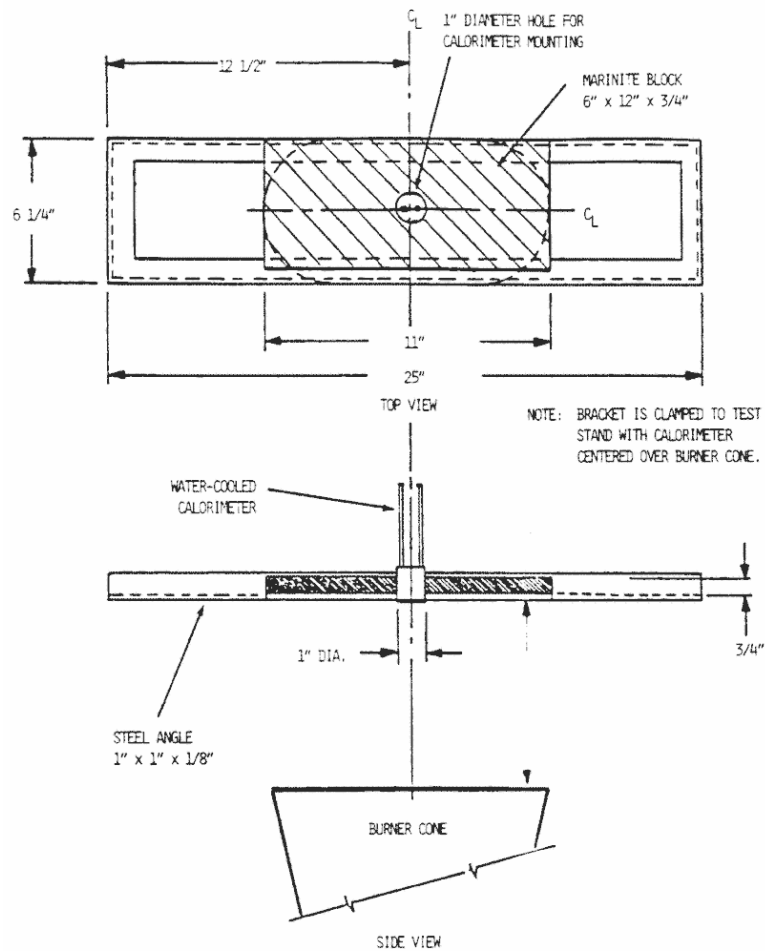
FIGURE 2. CALORIMETER BRACKET
