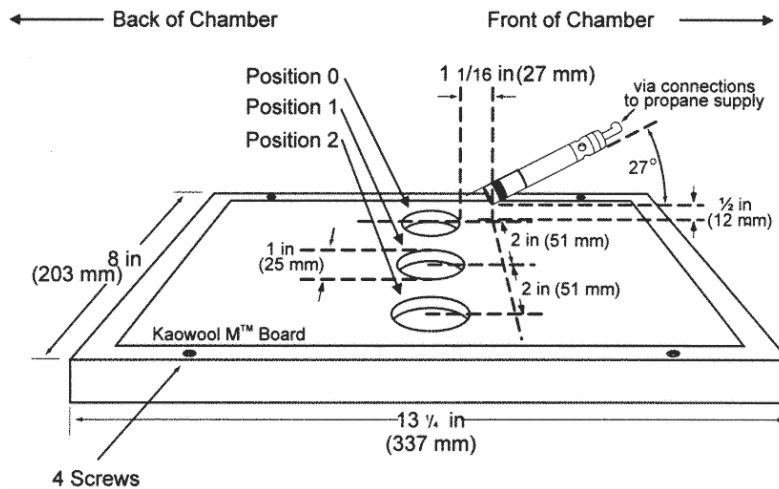
Figure 7 - Calorimeter Holding Frame
