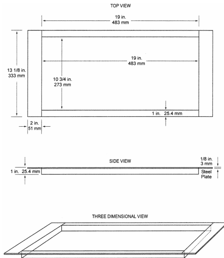
Figure 5: 3 views
