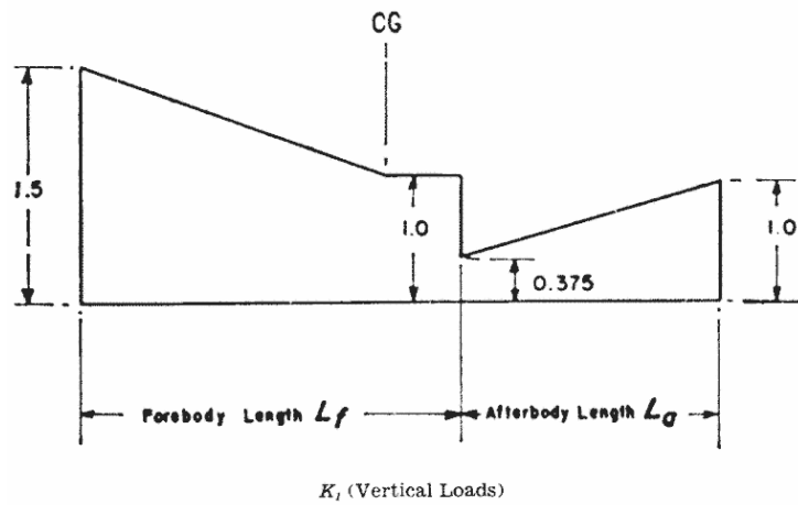
FIGURE 2—Hull station weighing factor.
