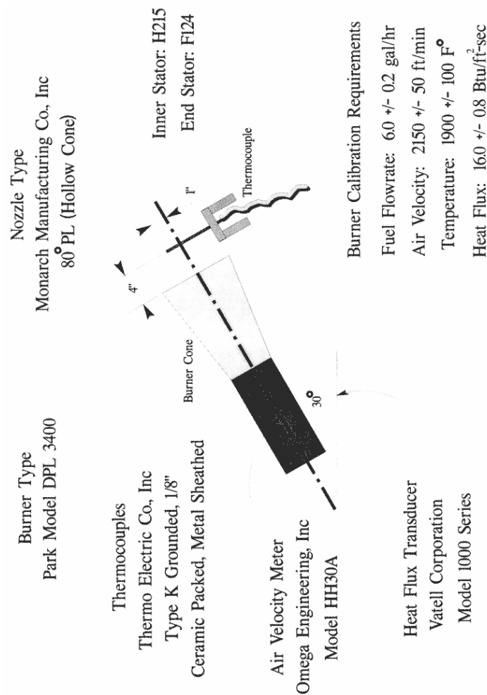
Figure 8 – Burner Information and Calibration Settings
