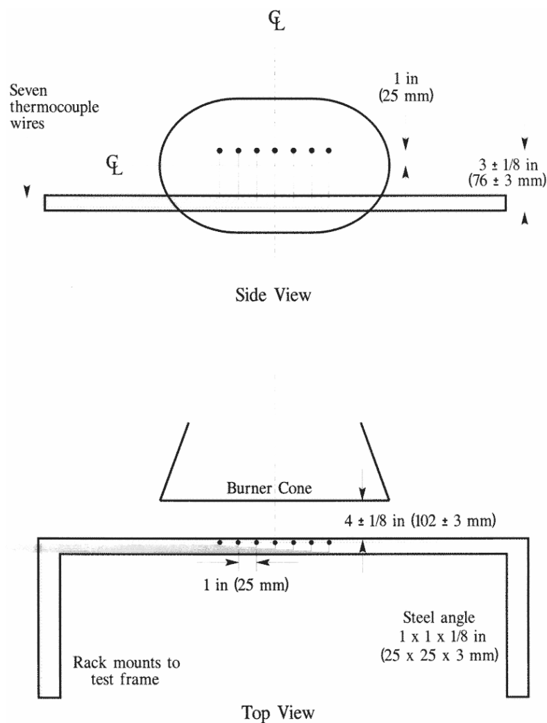
Figure 5 – Thermocouple Rake Position Relative to Burner Cone
