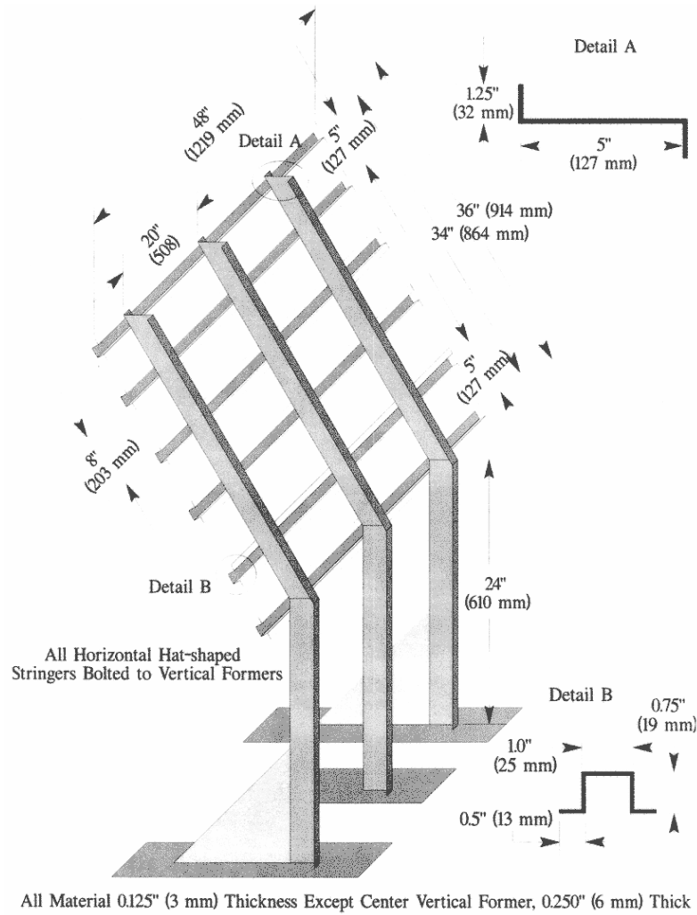
Figure 1 - Burnthrough Test Apparatus Specimen Holder
