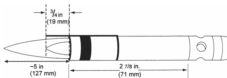
Figure 6 – Propane Pilot Burner
