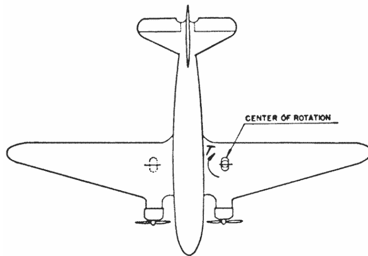
FIGURE 8—Pivoting, nose or tail wheel type.
