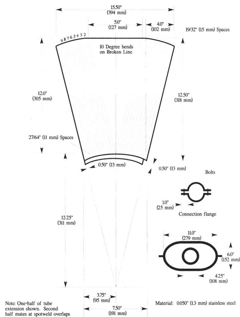
Figure 3 – Burner Draft Tube Extension Cone Diagram
