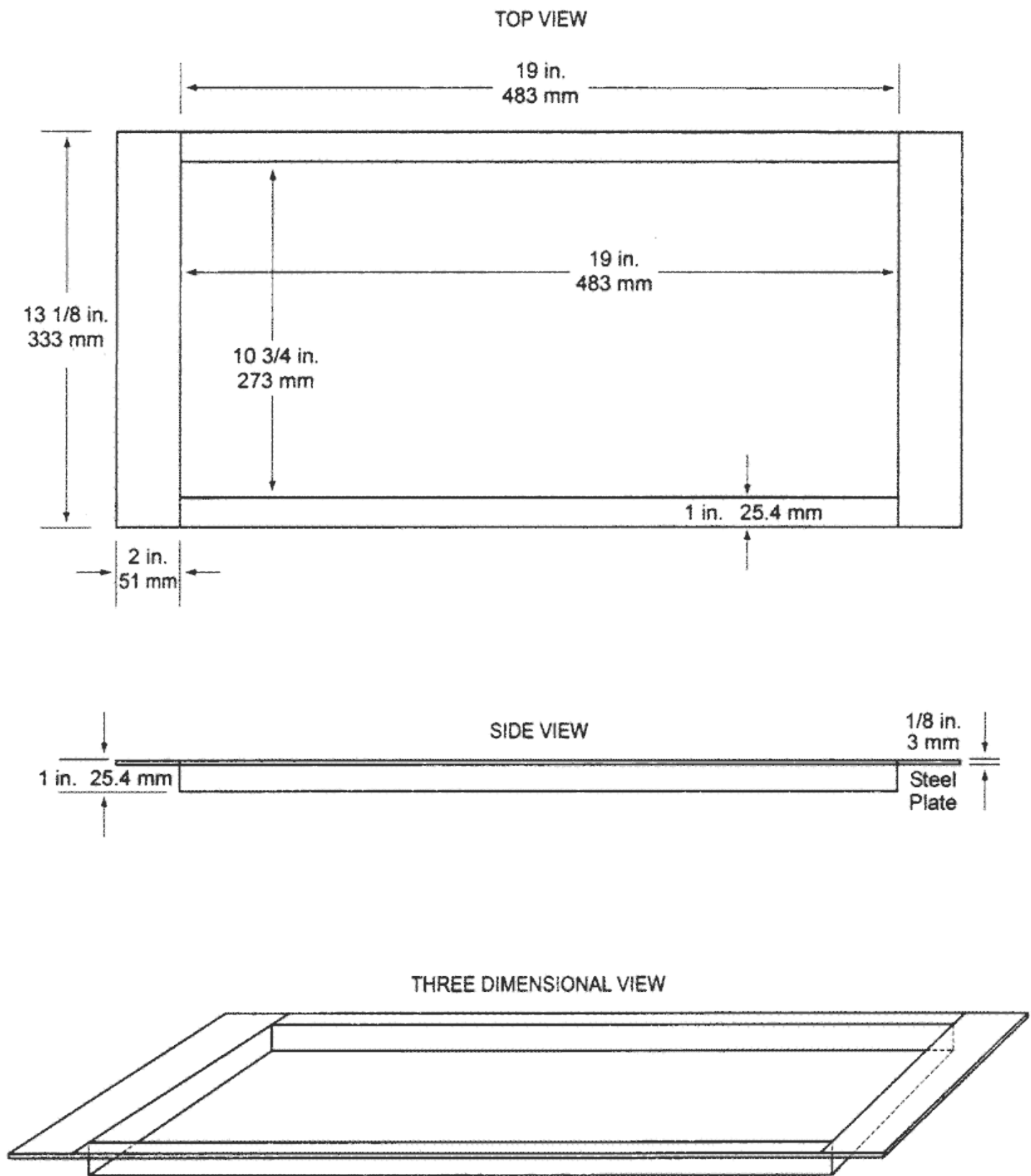
Figure 5: 3 views
