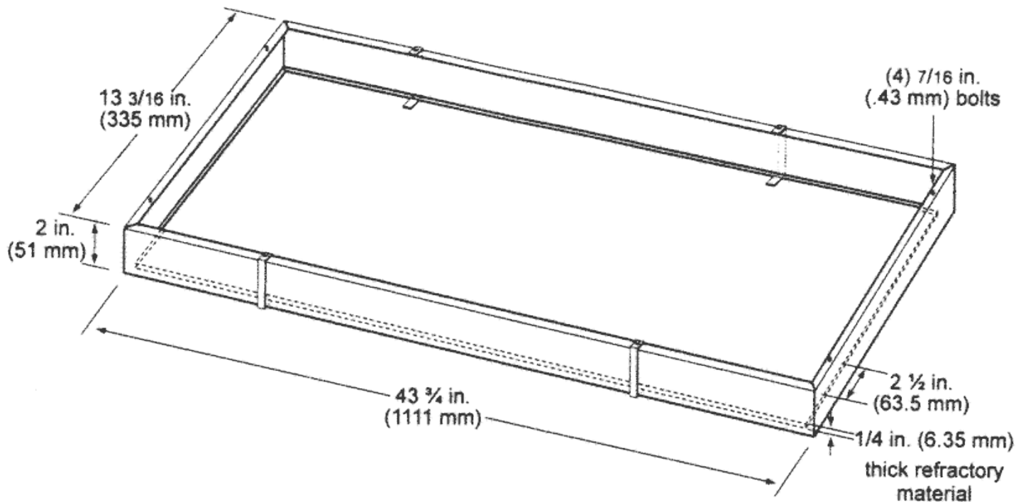
Figure 4 - Sliding Platform
