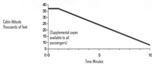
FIGURE 2—Cabin Altitude—Time History
