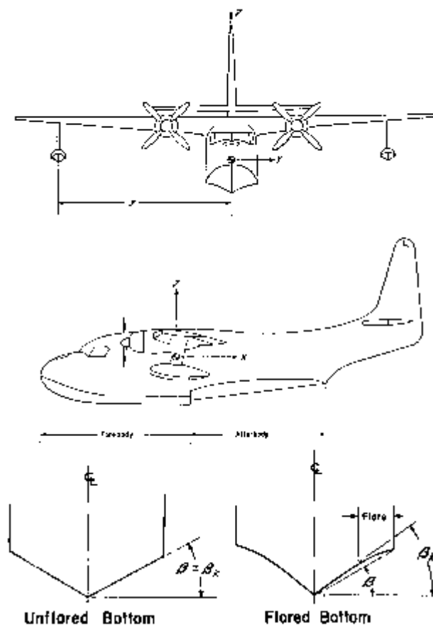
Appendix B Figure 1—Essential definition of angles, dimensions, and directions for a steepening
