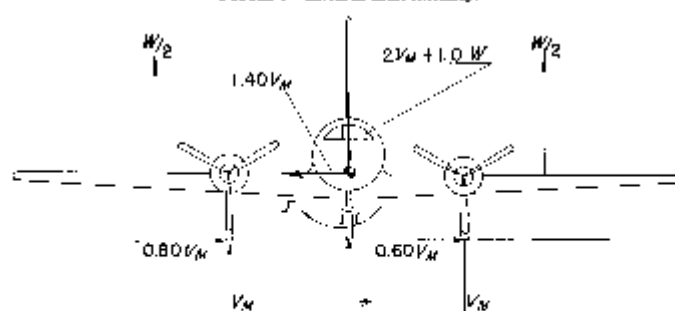
FIGURE 5—Lateral drift landing.
